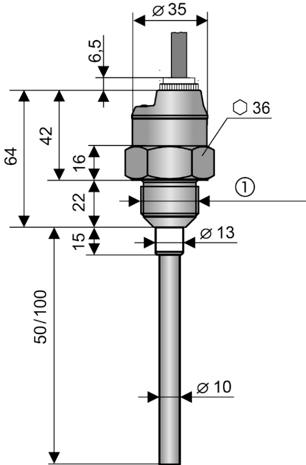
Dimensions (in mm) Process connection
