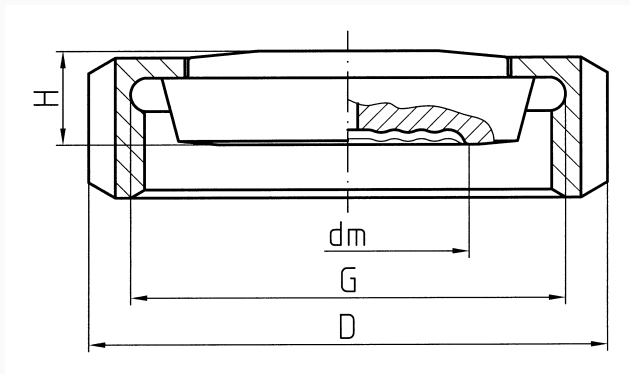
Tapered socket DIN 11851 type D/DIN 11887 type B with grooved union nut DIN 11851 type F
