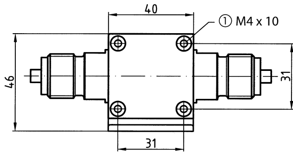
Dimensions (in mm) screw
