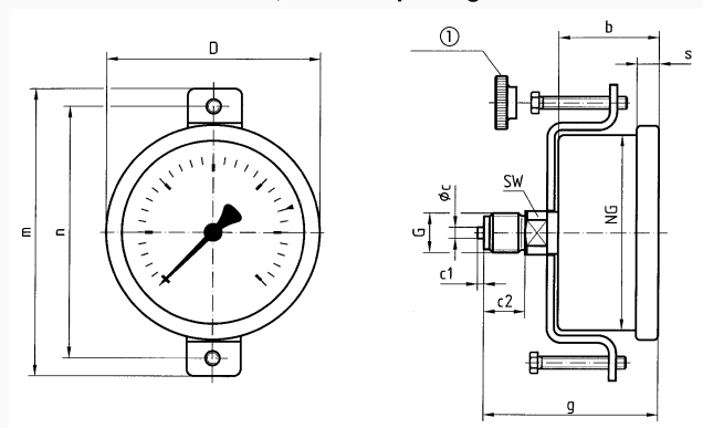
Dimensions (mm)
