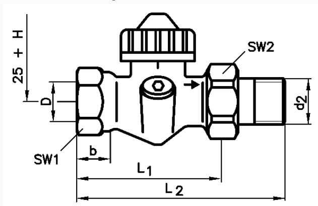
Types and dimensions as per EN 215, series D
