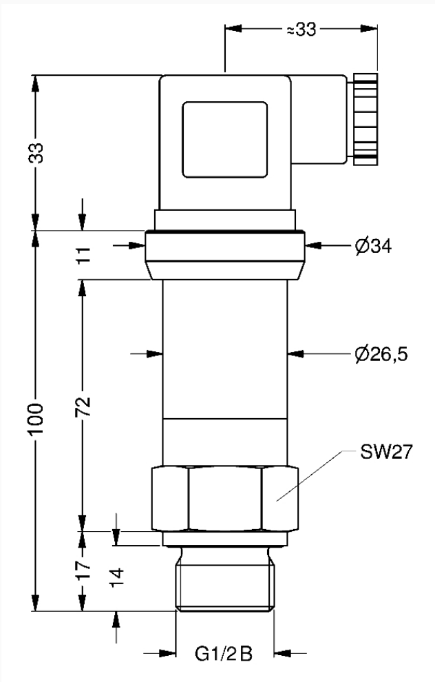
Dimensions (mm)
