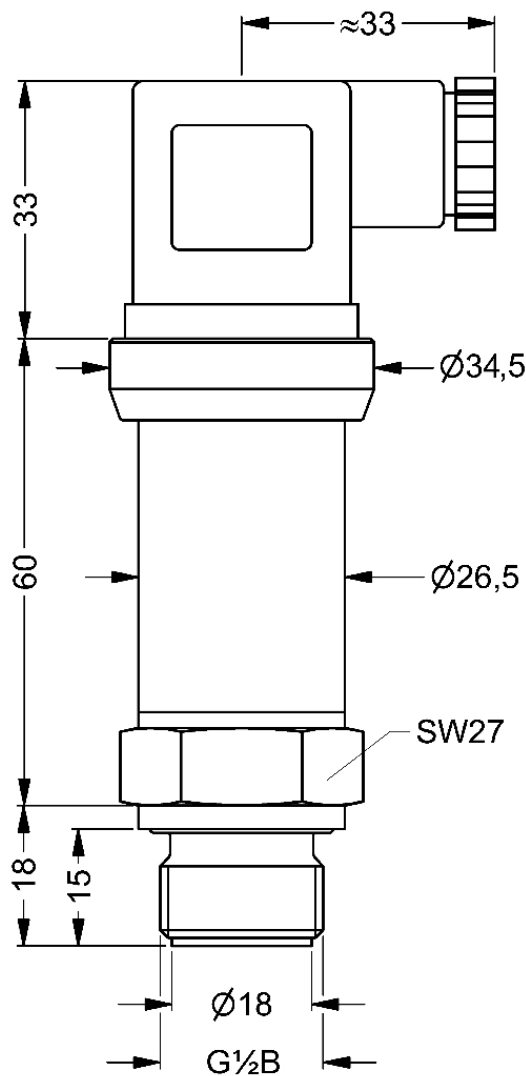
Dimensions (mm)
