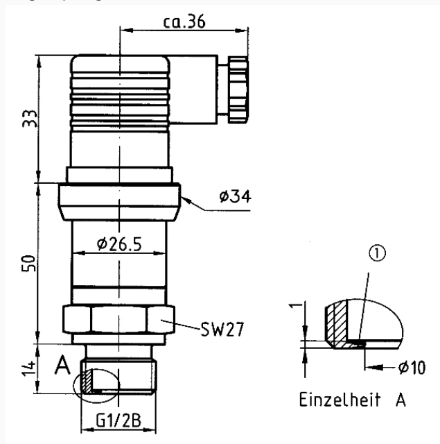
DMU 01 VM with connection G \frac{1}{2} B DIN 3852 type E with protruding diaphragm
